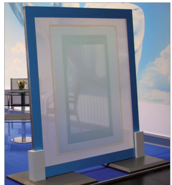
KOENEN precision screen XXL for the manufacture of dye-sensitised solar cells (in cooperation with the Fraunhofer ISE).
